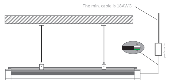
B : Screw the steel cable onto the ceiling
