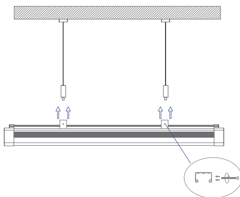
C : Hung the fixture under the steel cable and secure the fixture by steel cable
